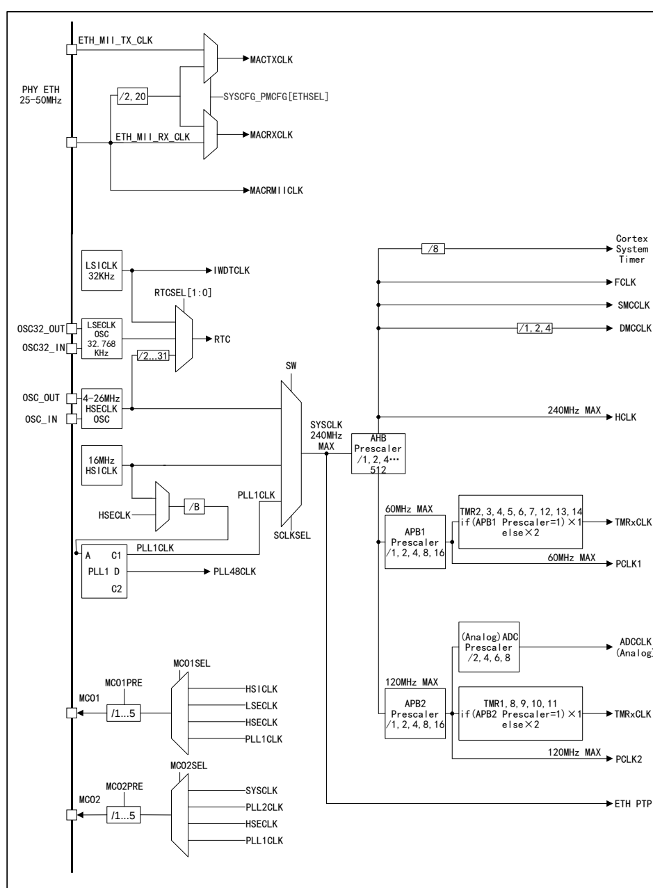
Figure 8 APM32F425xG_F427xG Clock Tree
