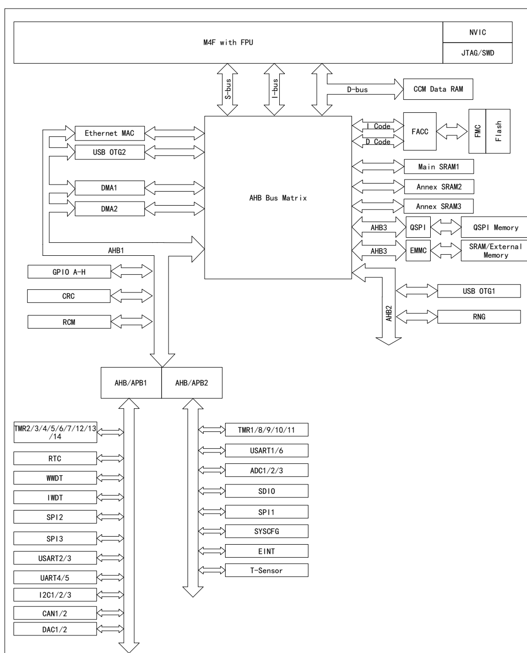
Figure 7 APM32F425xG_F427xG System Block Diagram
